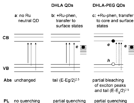
Figure 7. Schematic representation of the proposed model for charge transfer. (a) Absorption and PL spectra are unaffected for neutral QDs. (b) With DHLA QDs, charge transfer to QD surface states dominates the interactions and leads to partially quenched PL and a broad absorption tail. (c) With DHLA-PEG QDs, a combined transfer to surface states as well as core states leads to additional partial bleaching of the exciton absorption features along with quenching of the QD PL.
